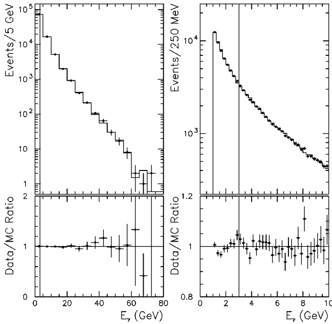
FIG. 3. Data-MC comparisons of the photon energy in the laboratory frame at two different scales. The photon energy was required to be above 3 GeV to be included in the K_{e3\gamma} sample. This cut is indicated by the vertical line in each plot. The \chi^2/\text{DOF} = 6.2/14 for the first plot and 24.4/27 for the second.
