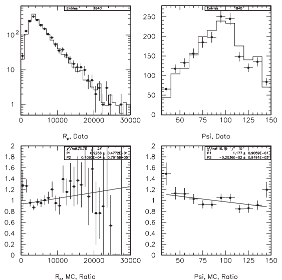
Figure 1. Data/MC comparisons of r_p and \psi .
