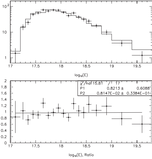
Figure 2. Data/MC comparison of reconstructed energies.
