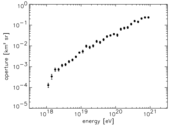
FIG. 2.— Calculated HiRes-II electron-neutrino aperture.
