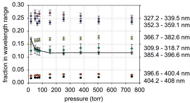
Fig. 5. Pressure variation of the relative contributions of various spectral ranges.
