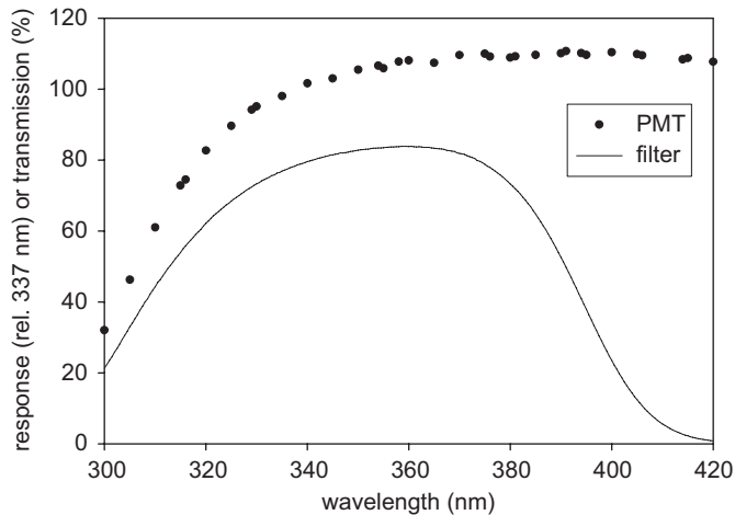
Fig. 4. PMT response relative to that at 337 nm, and transmission of HiRes filter, vs. wavelength.
