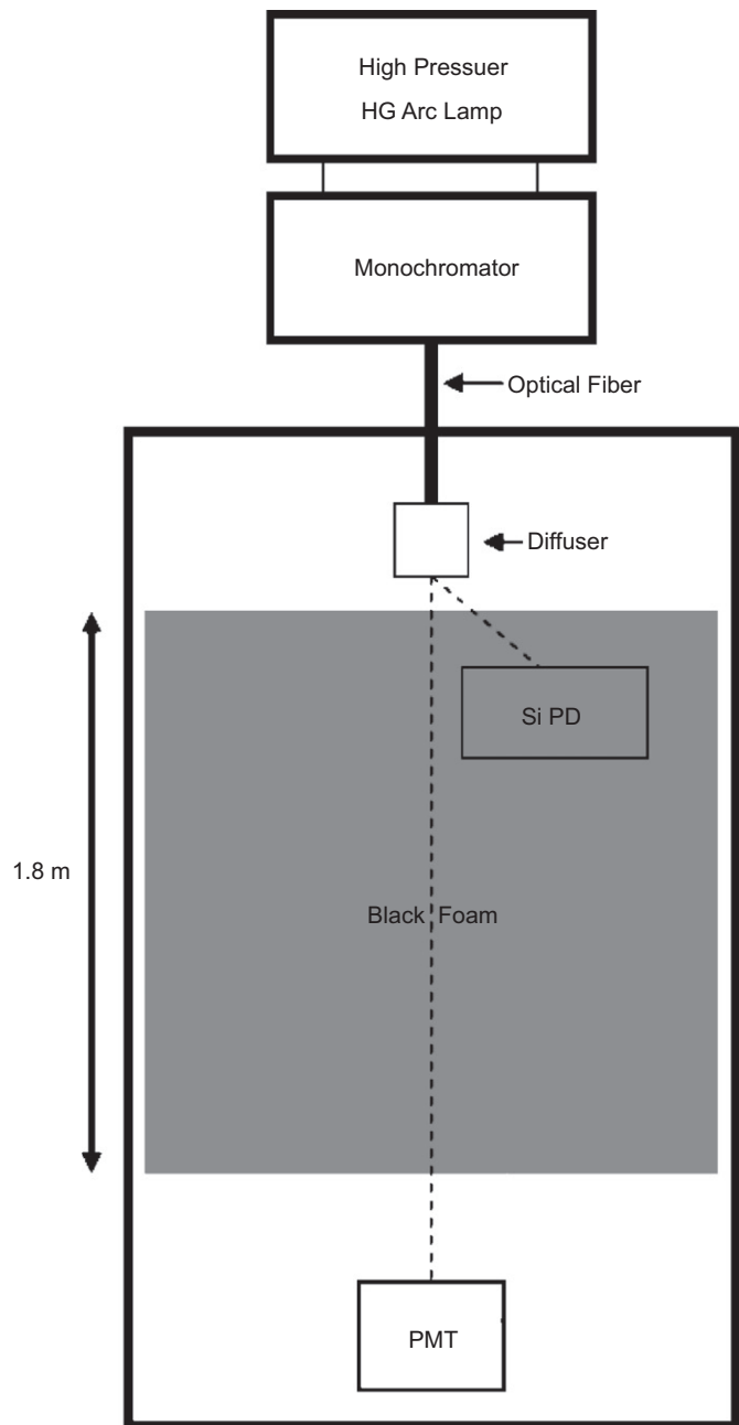
Fig. 3. The relative calibration setup. See text for details.
