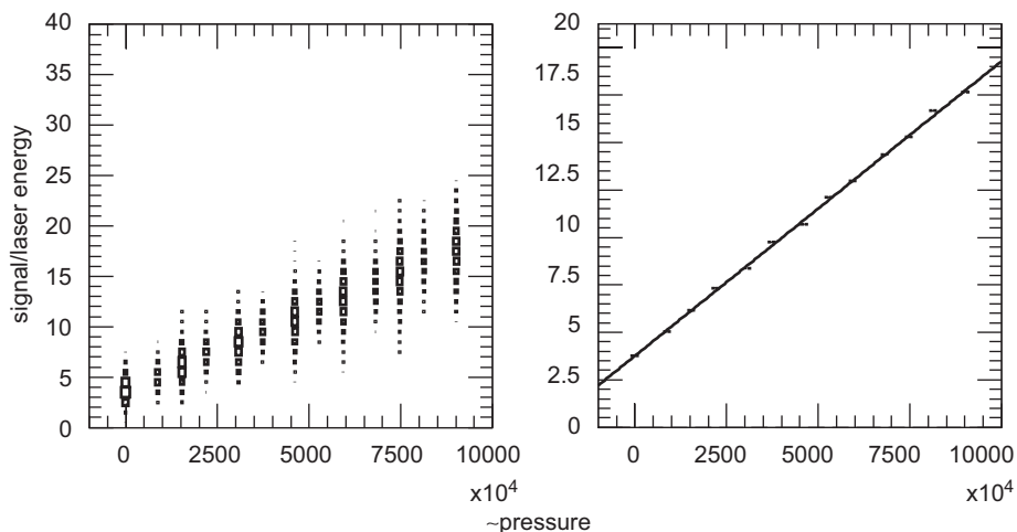
Fig. 2. PMT response against Rayleigh scattering intensity, controlled by changing air pressure. The plots represent Eq. (1). The left plot shows the scattering of the data during each of the pressure runs. The right plot shows the fit to the mean values of each run.
