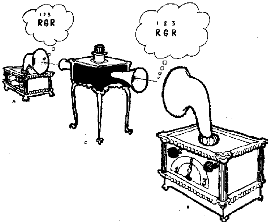
Figure 7 – Instruction sets.
